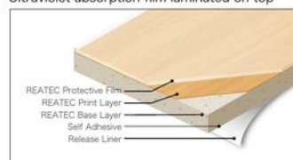
Ultraviolet absorption film laminated on top
